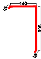
Gable Flashing Code : GF405
