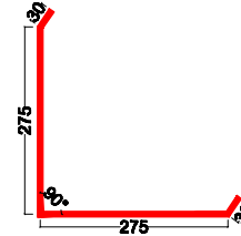
Corner Flashing Code : CF610
