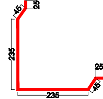
Profiled Corner Flashing Code : PCF610
